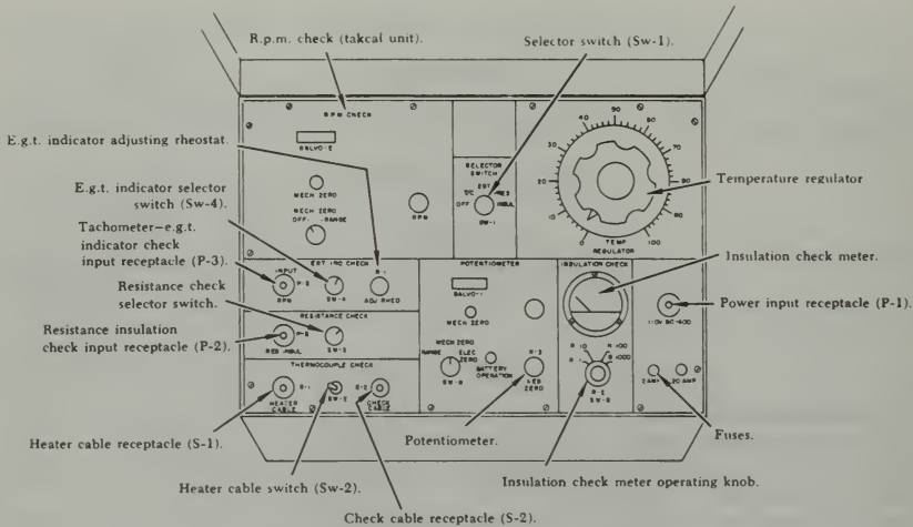
FIGURE 10-71. Jetcal analyzer instrument compartment.
